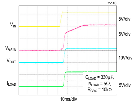
STARTUP BEHAVIOR
