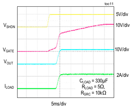
EXITING SHUTDOWN
