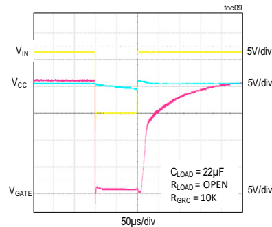
MICROCUT OPERATION
