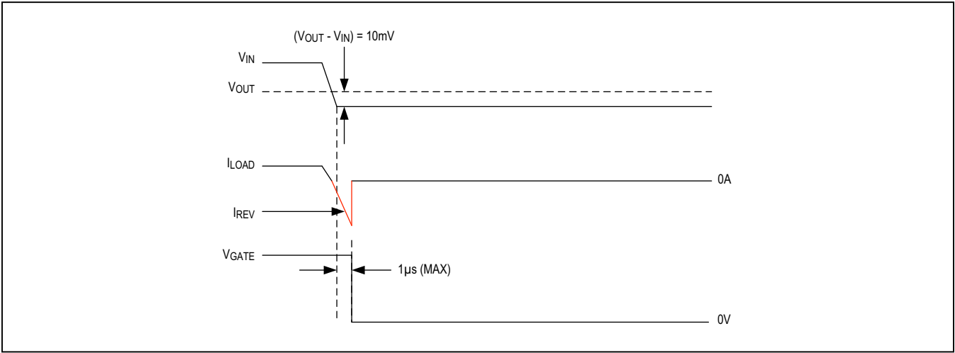
Figure 3. Reverse-Voltage Fault
